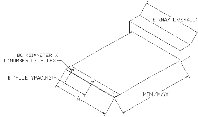
ENCLOSED STYLE
